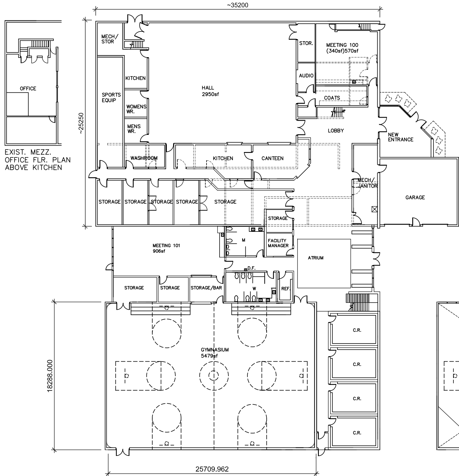
MAIN LEVEL
